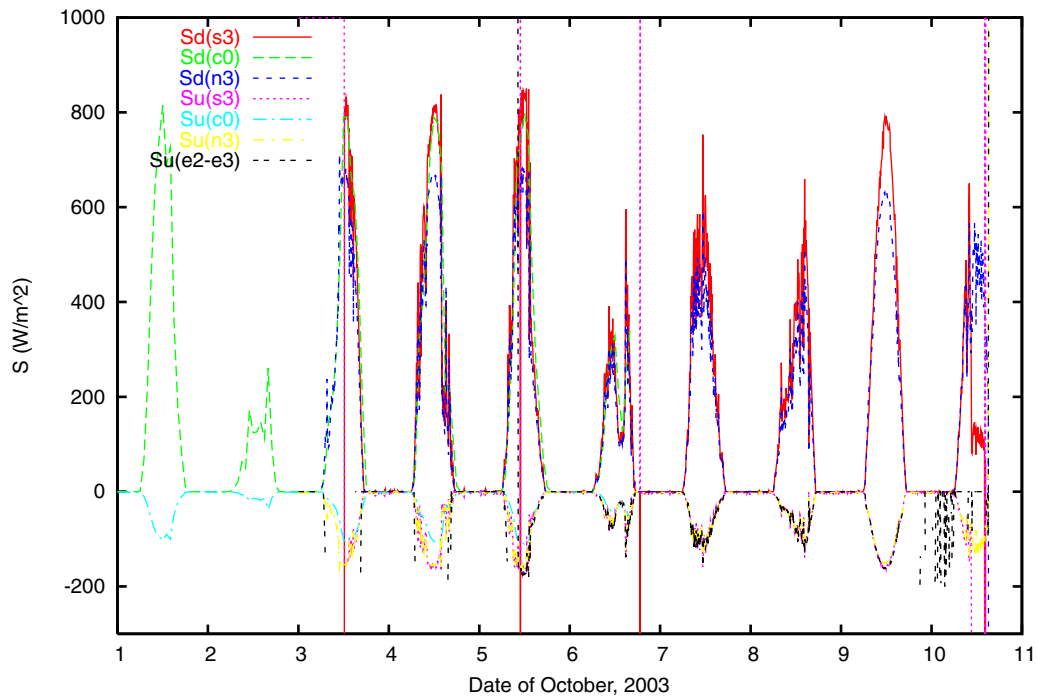
S_down &amp; S_up
