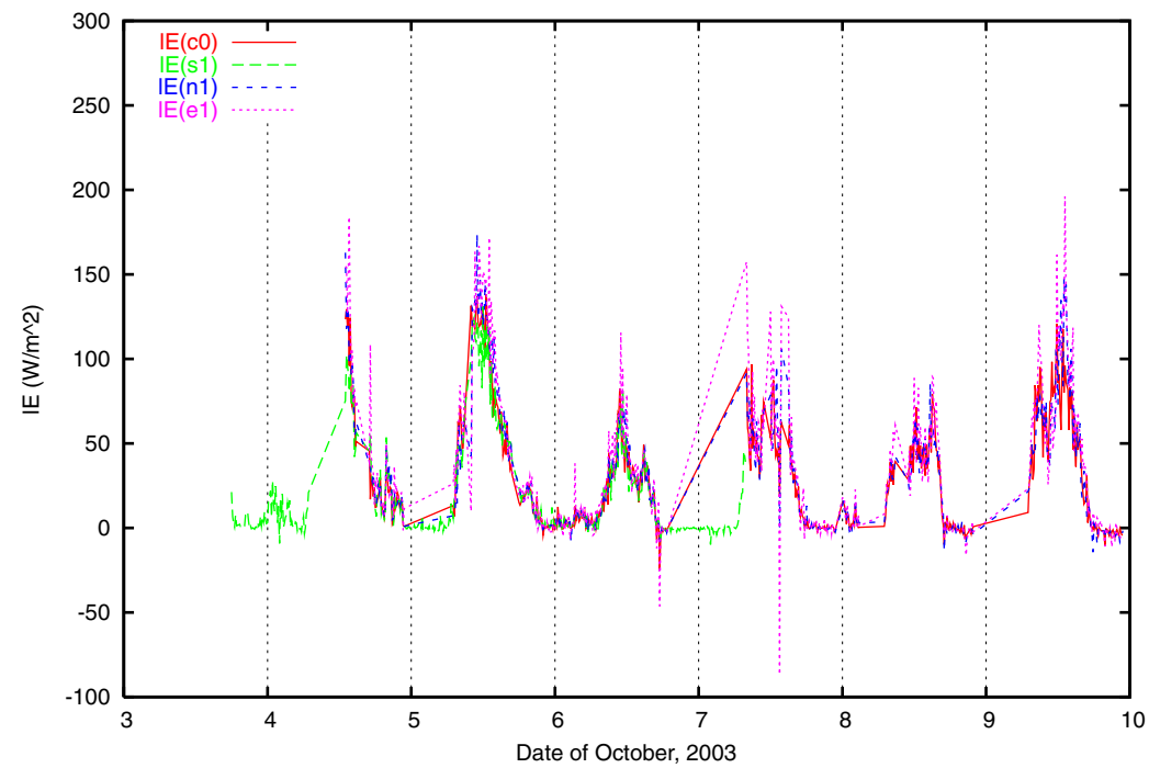
Latent Heat Flux
