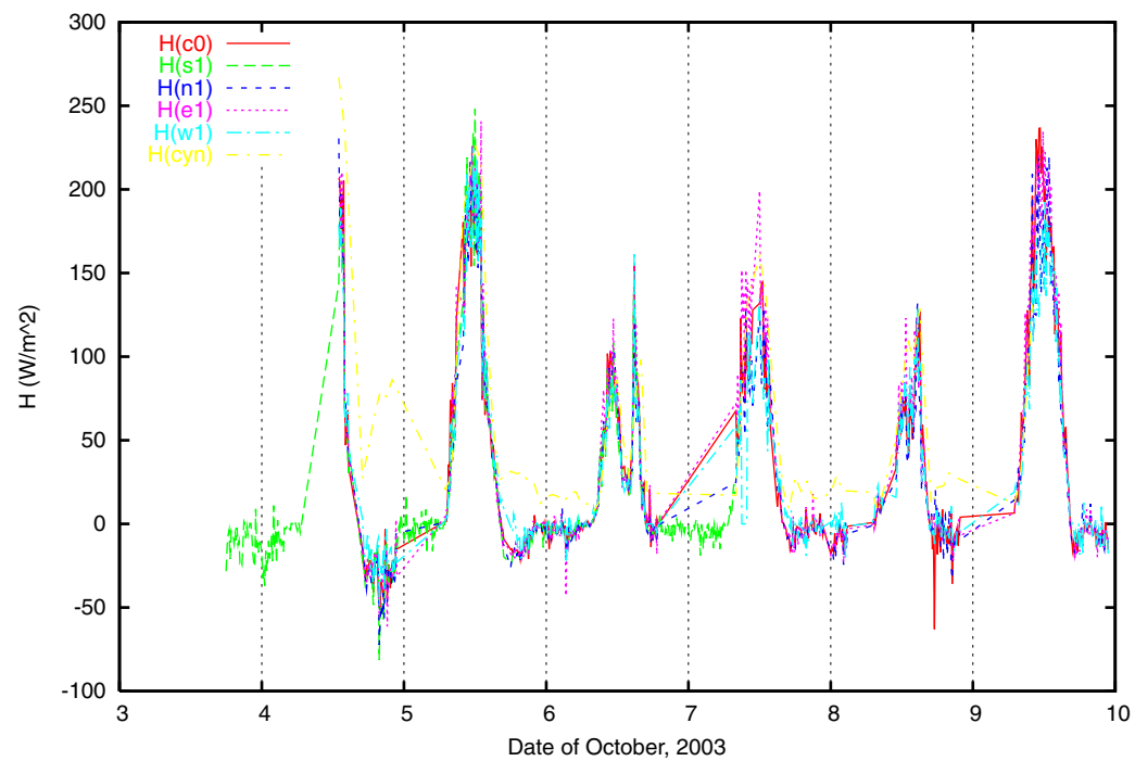
Sensible Heat Flux
