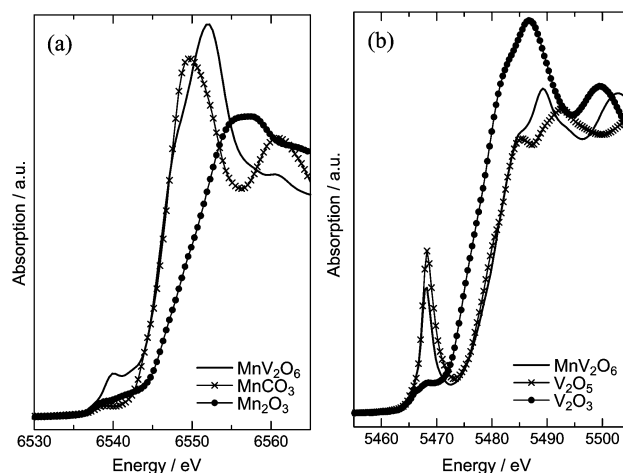
Fig. 2 XANES spectra of (a) Mn K-edge for \text{MnV}_2\text{O}_6 , \text{MnCO}_3 and \text{Mn}_2\text{O}_3 , (b) V K-edge for \text{MnV}_2\text{O}_6 , \text{V}_2\text{O}_3 and \text{V}_2\text{O}_5 .
